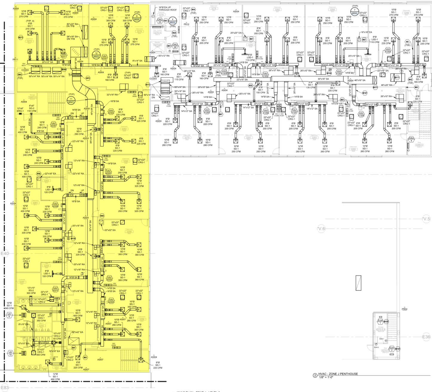
① HVAC PLAN - ZONE J - LEVEL 3 1/8" = 1'-0"
